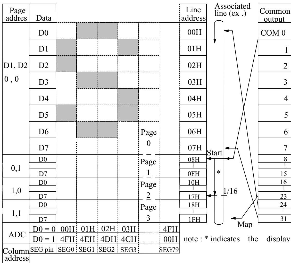
Figure 2 : Display Data RAM Addressing
